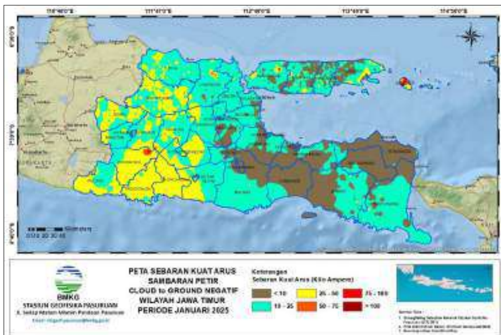
Gambar 14. Peta Kuat Arus Sambaran Petir Cloud to Ground Negatif (CG-)
