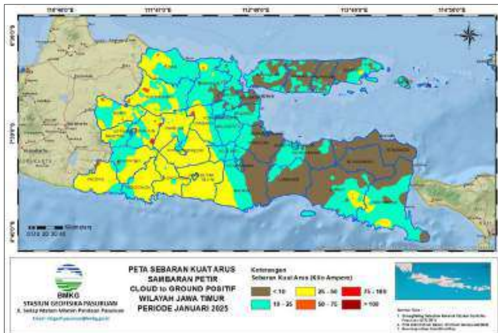
Gambar 12. Peta Kuat Arus Sambaran Petir Cloud to Ground Positif ( CG+ )
