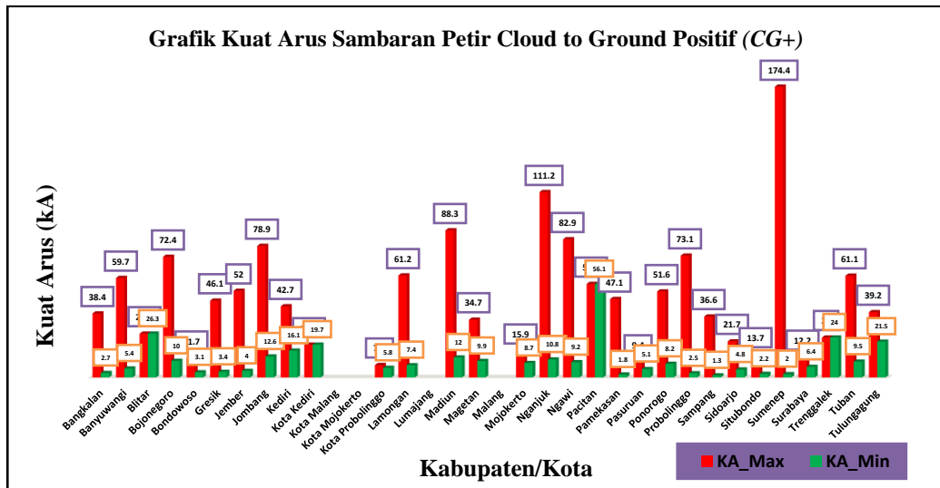
Gambar 13. Grafik Kuat Arus Sambaran Petir Cloud to Ground Positif (CG+)
